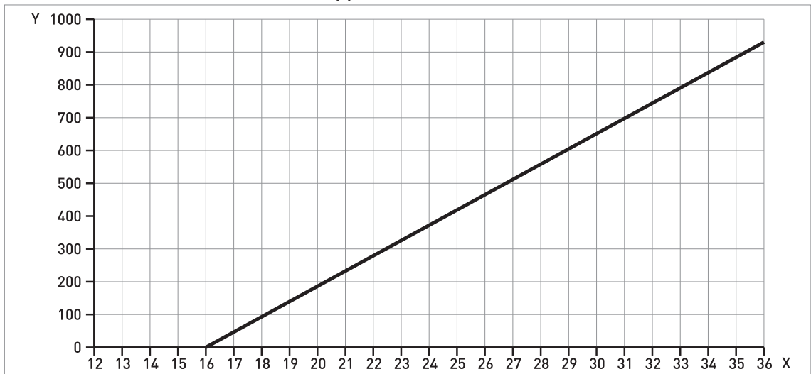
Figure 2-6: Minimum power supply voltage for an output of 21.5 mA at the terminals (Hazardous Location approval [Ex d / XP/NI])
